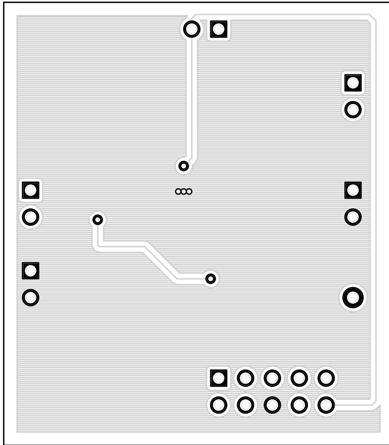
Figure 9. Bottom Layer Routing
